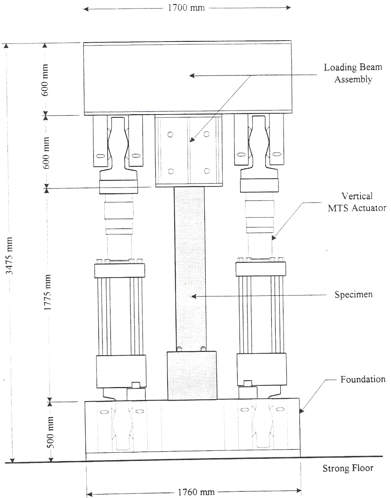
Fig. 14 Front Elevation of the Test Setup
