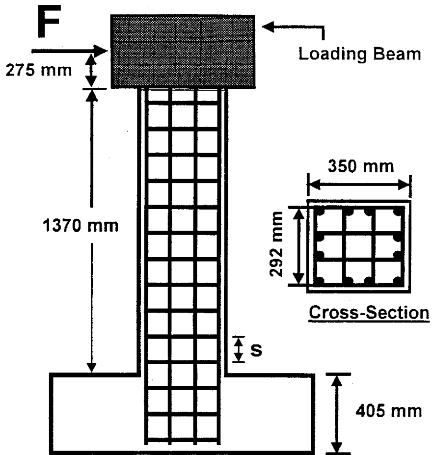
Fig. 1 Geometry of Column Specimens
