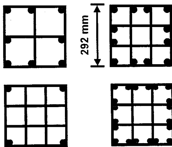
Fig. 2 Cross-Sectional Arrangements used in Columns
