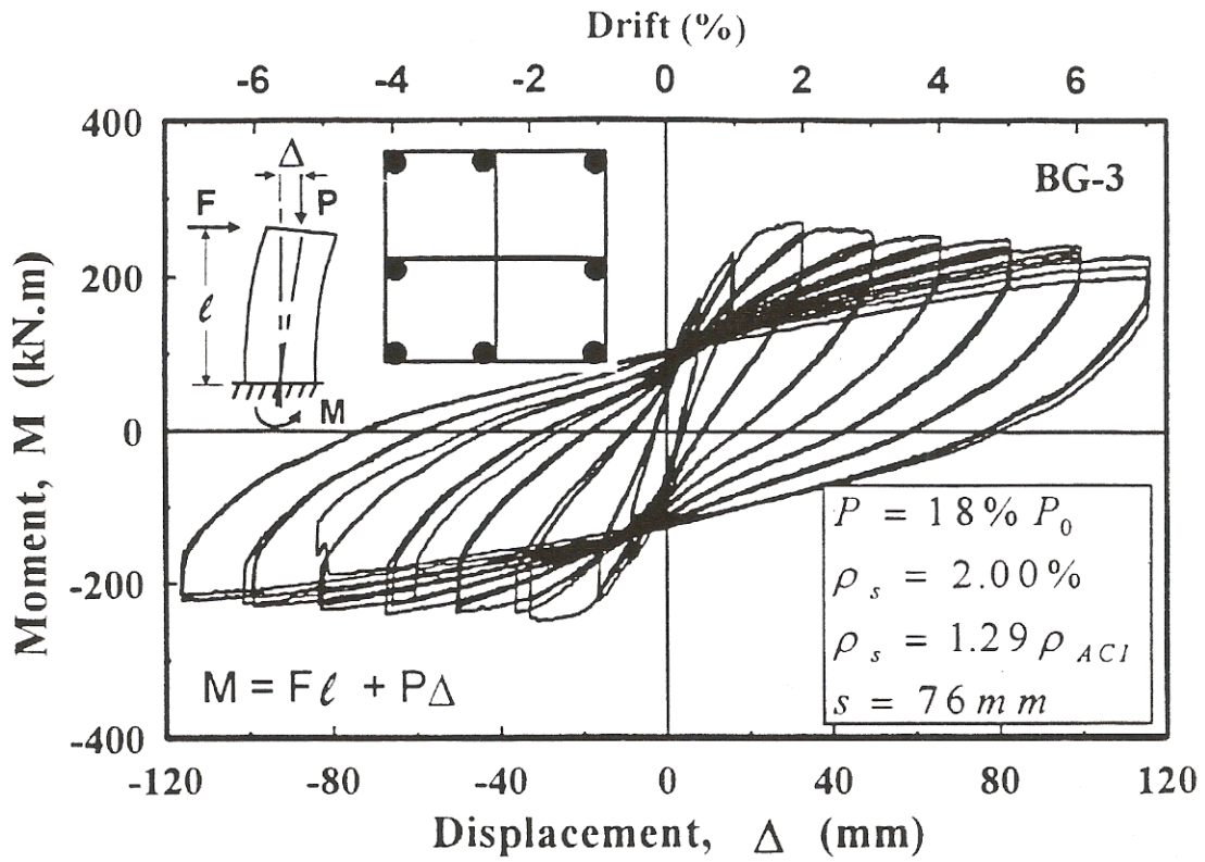
Fig. 23 Hysteretic Moment-Displacement Relationship for Column BG-3
