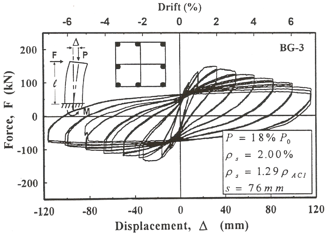
Fig. 24 Hysteretic Force-Displacement Relationship for Column BG-3
